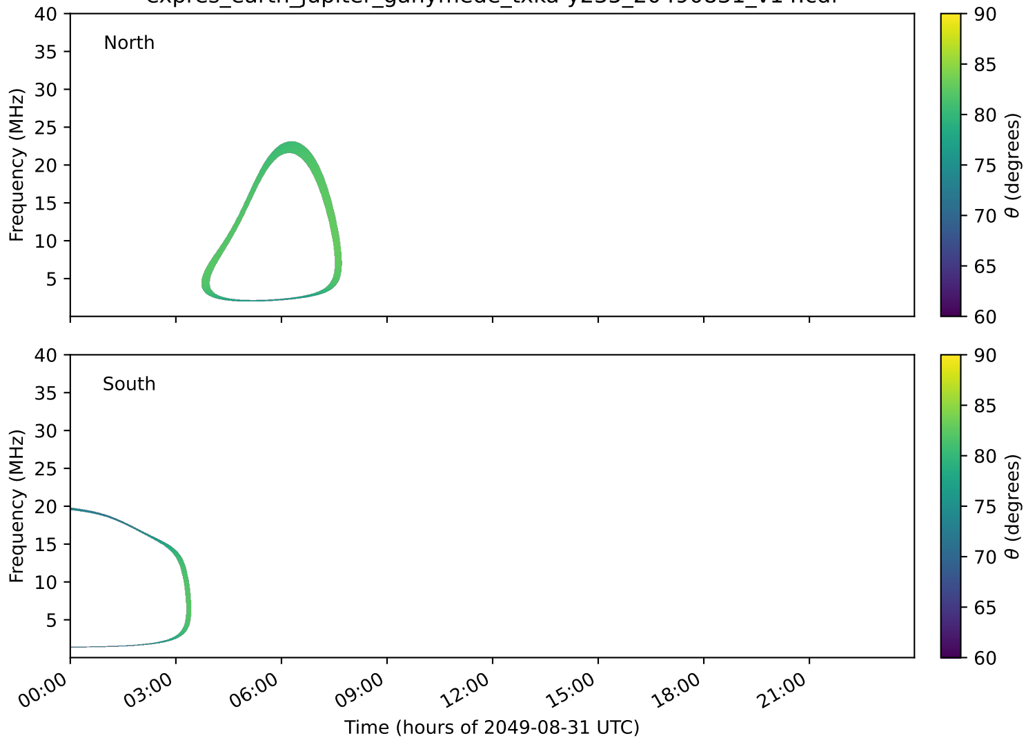
expres_earth_jupiter_ganymede_txka-y235_20490831_v14.cdf
