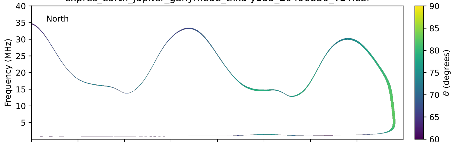
expres_earth_jupiter_ganymede_txka-y235_20490830_v14.cdf
