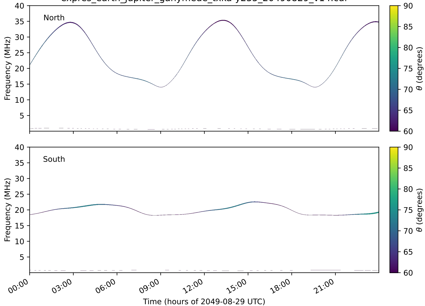
expres_earth_jupiter_ganymede_txka-y235_20490829_v14.cdf
