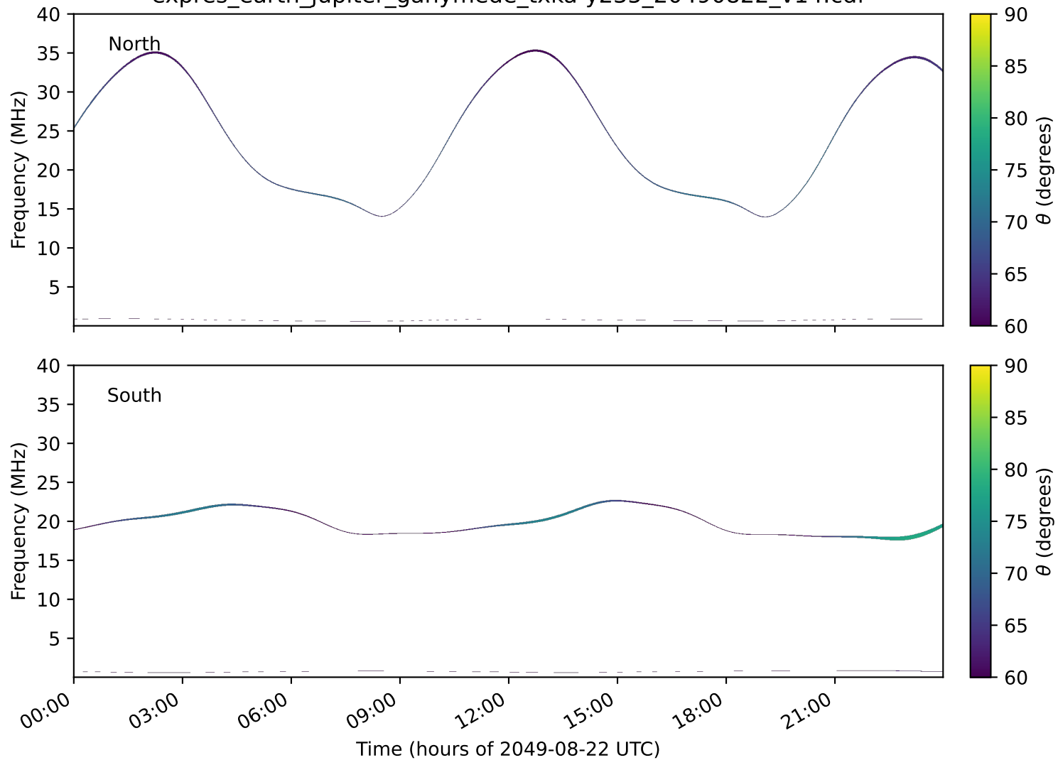
expres_earth_jupiter_ganymede_txka-y235_20490822_v14.cdf
