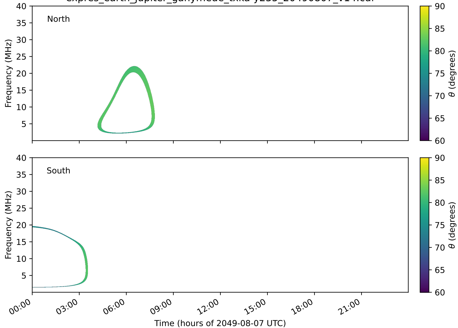
expres_earth_jupiter_ganymede_txka-y235_20490807_v14.cdf
