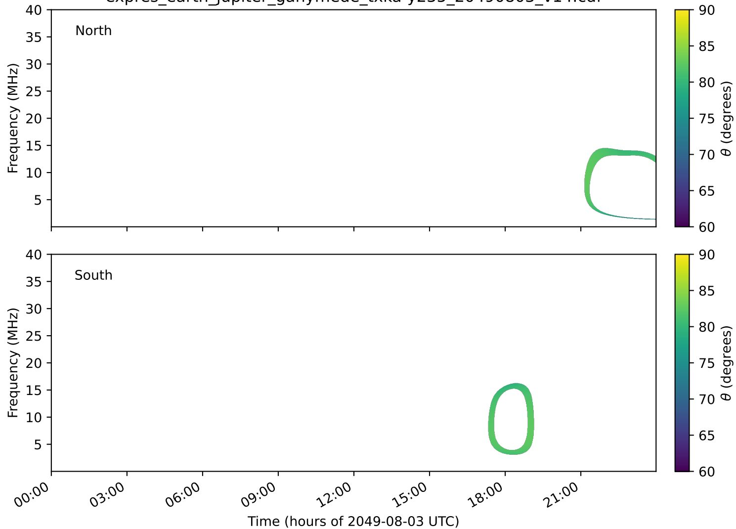
expres_earth_jupiter_ganymede_txka-y235_20490803_v14.cdf
