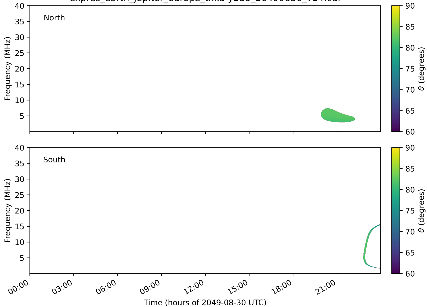
expres_earth_jupiter_europa_txka-y235_20490830_v14.cdf
