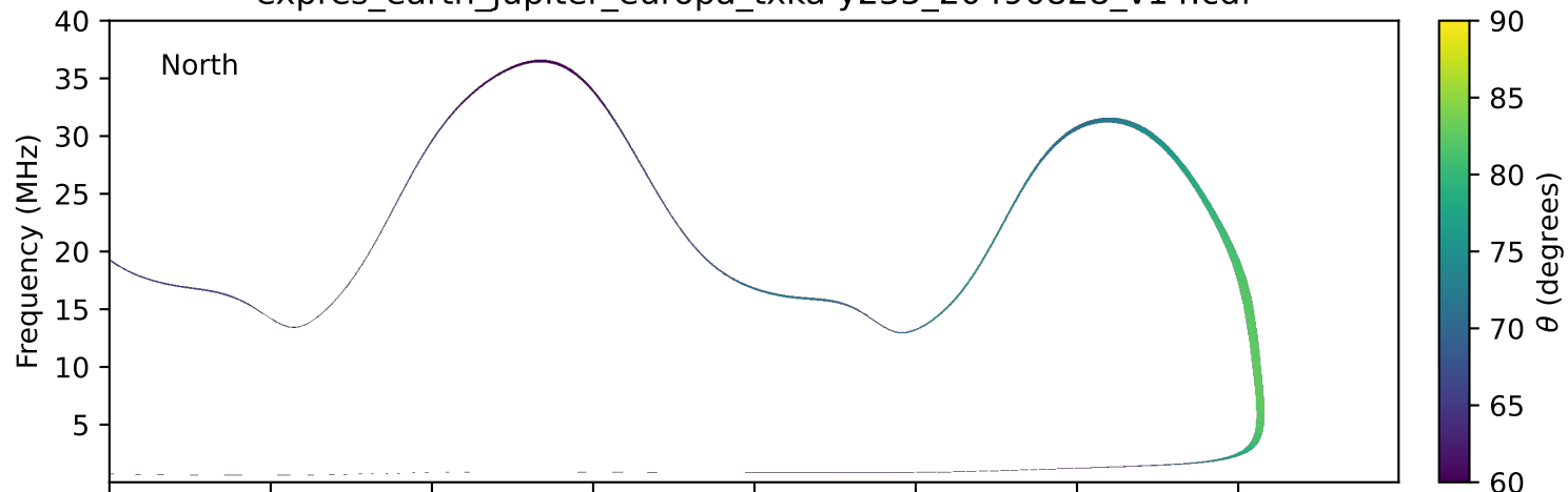
expres_earth_jupiter_europa_txka-y235_20490828_v14.cdf
