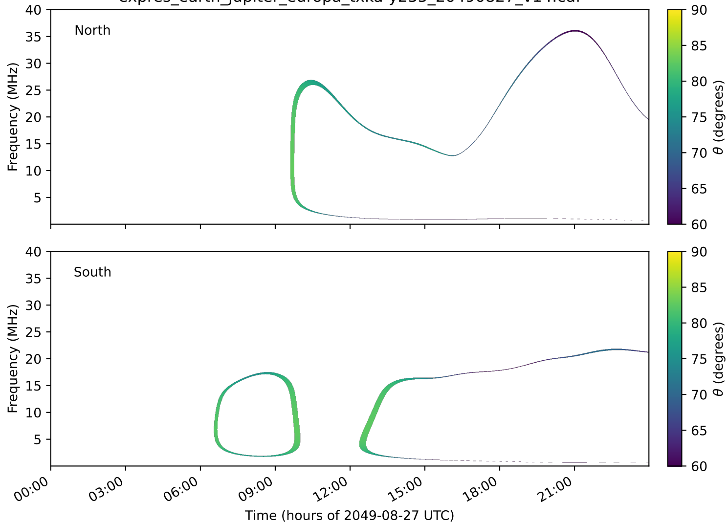
expres_earth_jupiter_europa_txka-y235_20490827_v14.cdf
