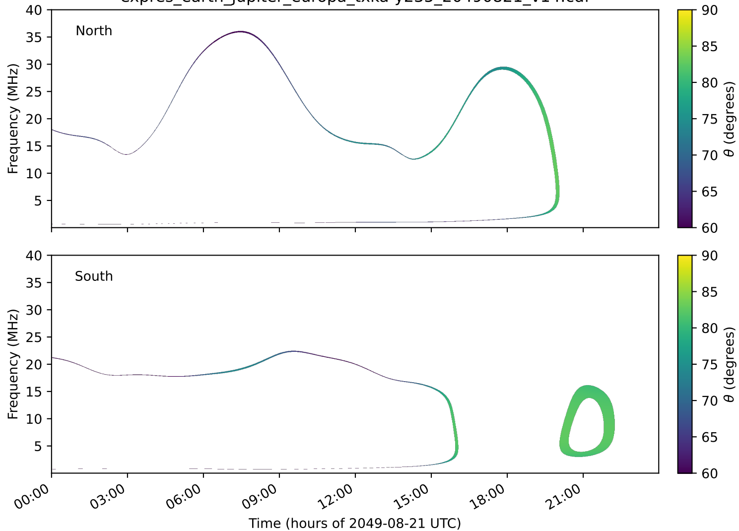
expres_earth_jupiter_europa_txka-y235_20490821_v14.cdf
