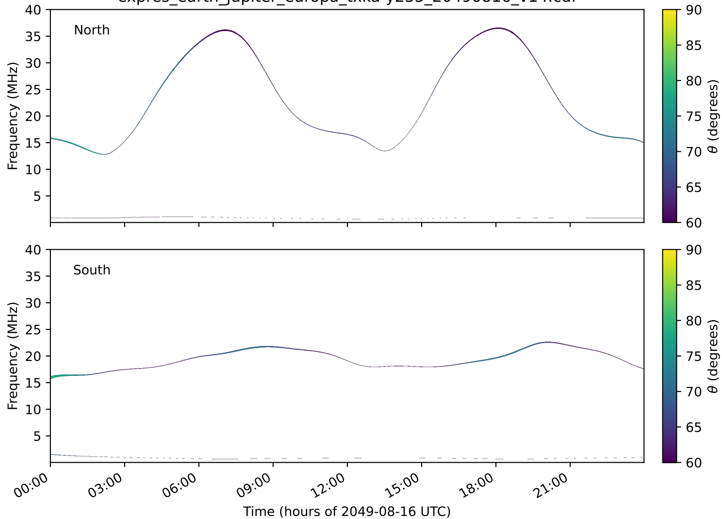
expres_earth_jupiter_europa_txka-y235_20490816_v14.cdf
