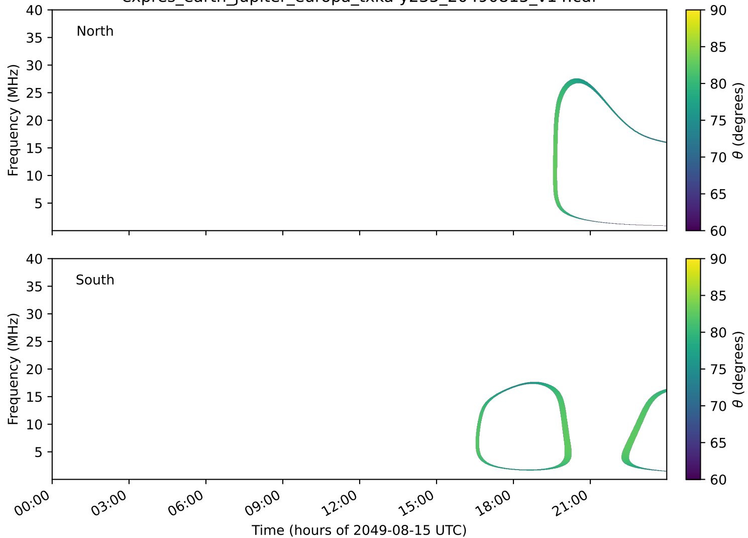
expres_earth_jupiter_europa_txka-y235_20490815_v14.cdf
