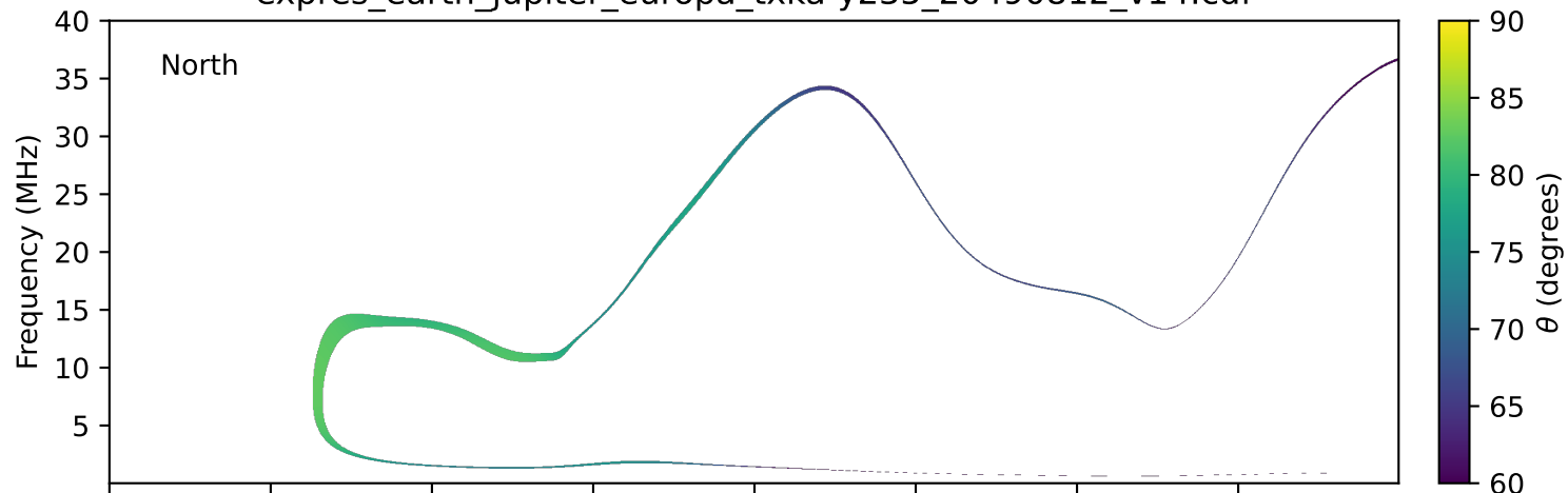
expres_earth_jupiter_europa_txka-y235_20490812_v14.cdf
