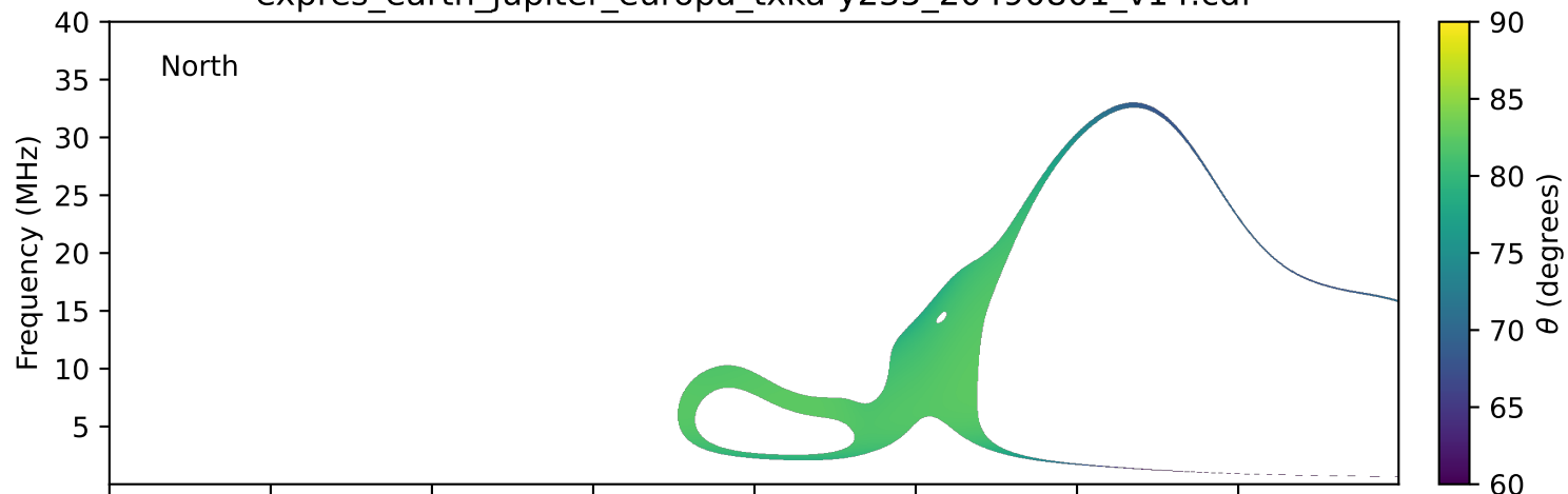
expres_earth_jupiter_europa_txka-y235_20490801_v14.cdf
