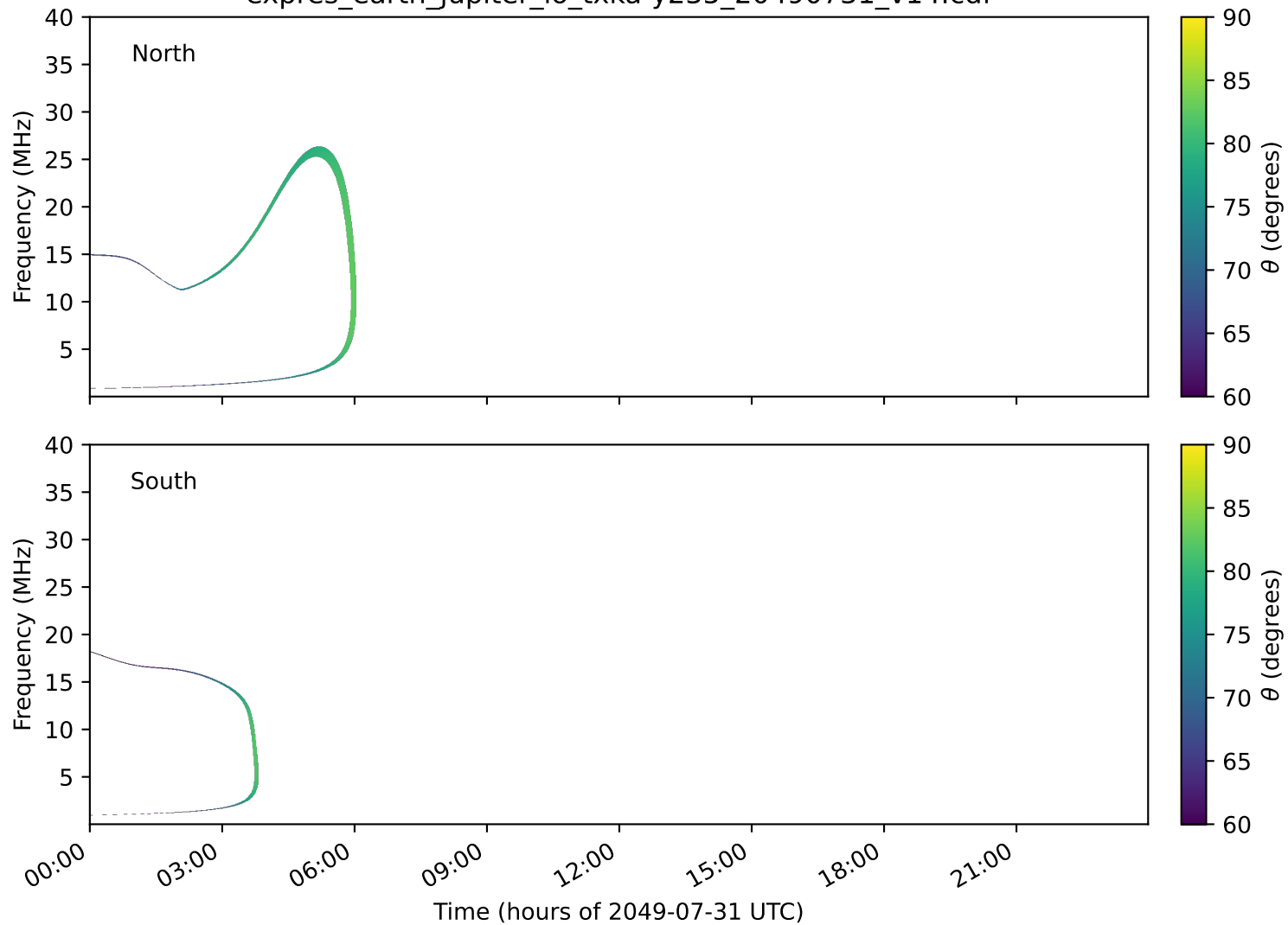
expres_earth_jupiter_io_txka-y235_20490731_v14.cdf
