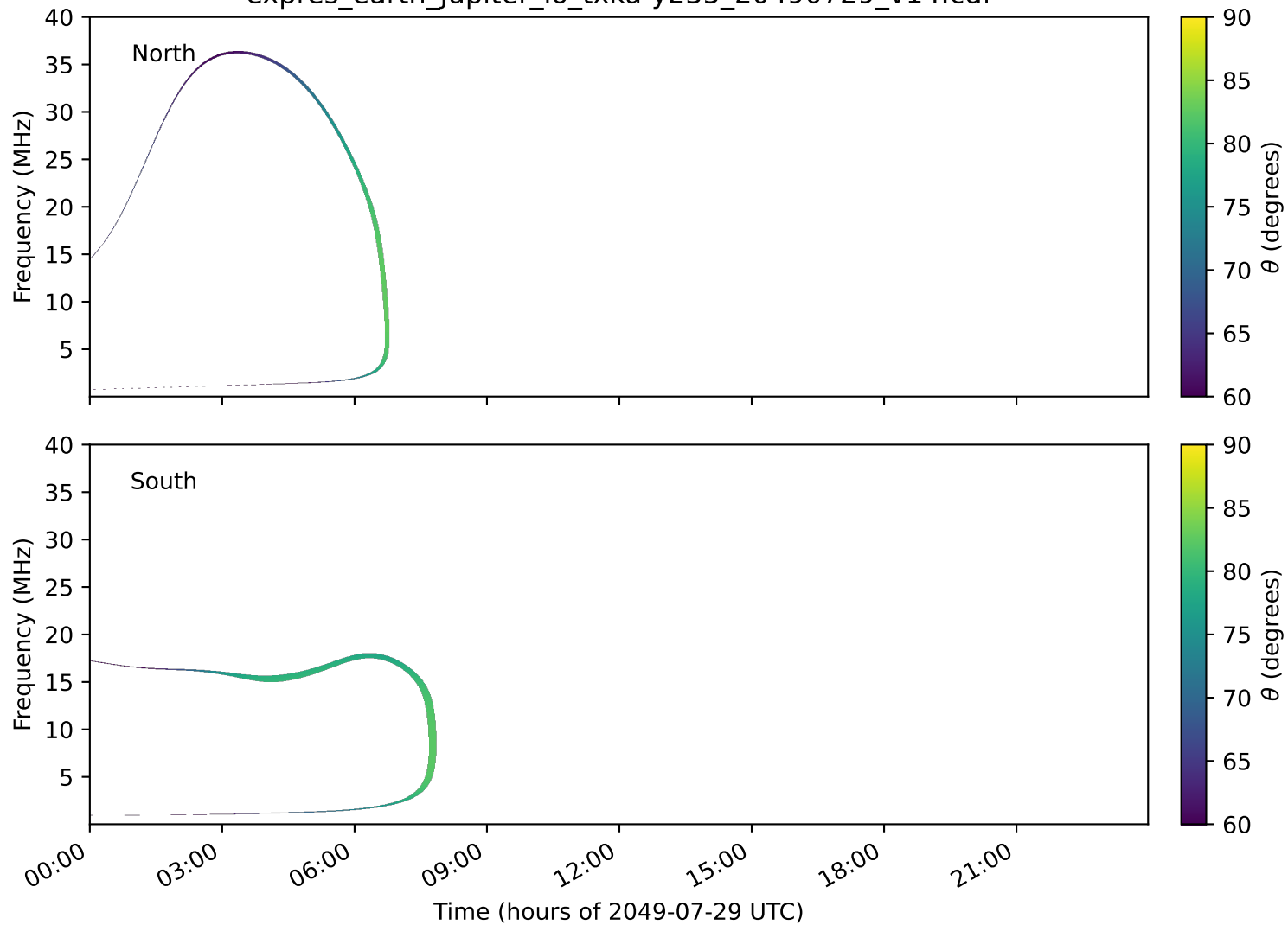
expres_earth_jupiter_io_txka-y235_20490729_v14.cdf
