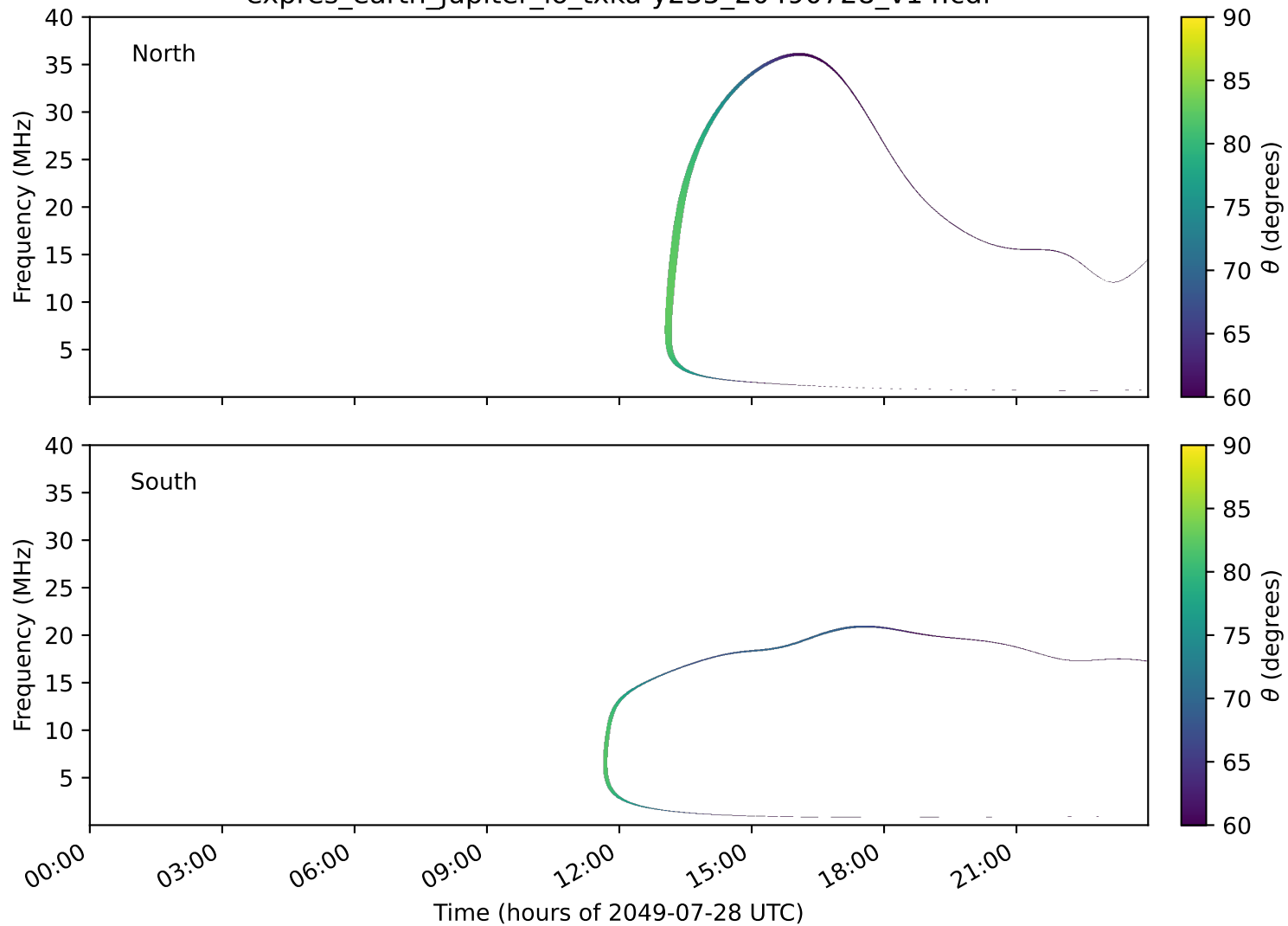
expres_earth_jupiter_io_txka-y235_20490728_v14.cdf
