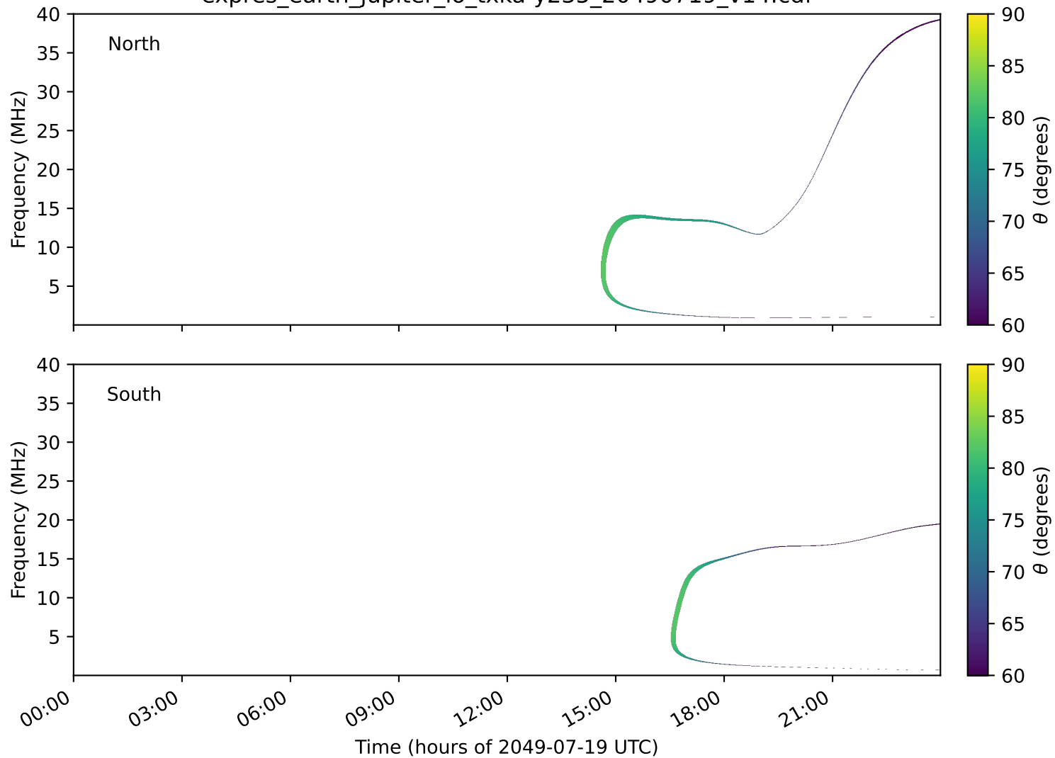
expres_earth_jupiter_io_txka-y235_20490719_v14.cdf
