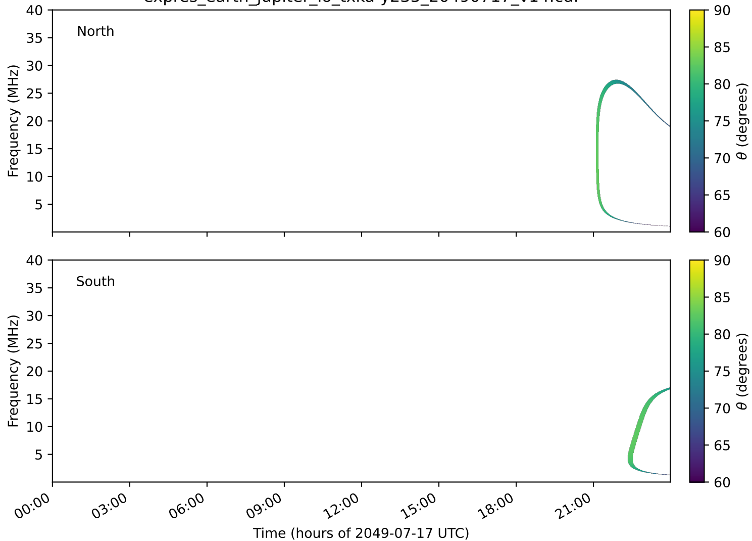
expres_earth_jupiter_io_txka-y235_20490717_v14.cdf
