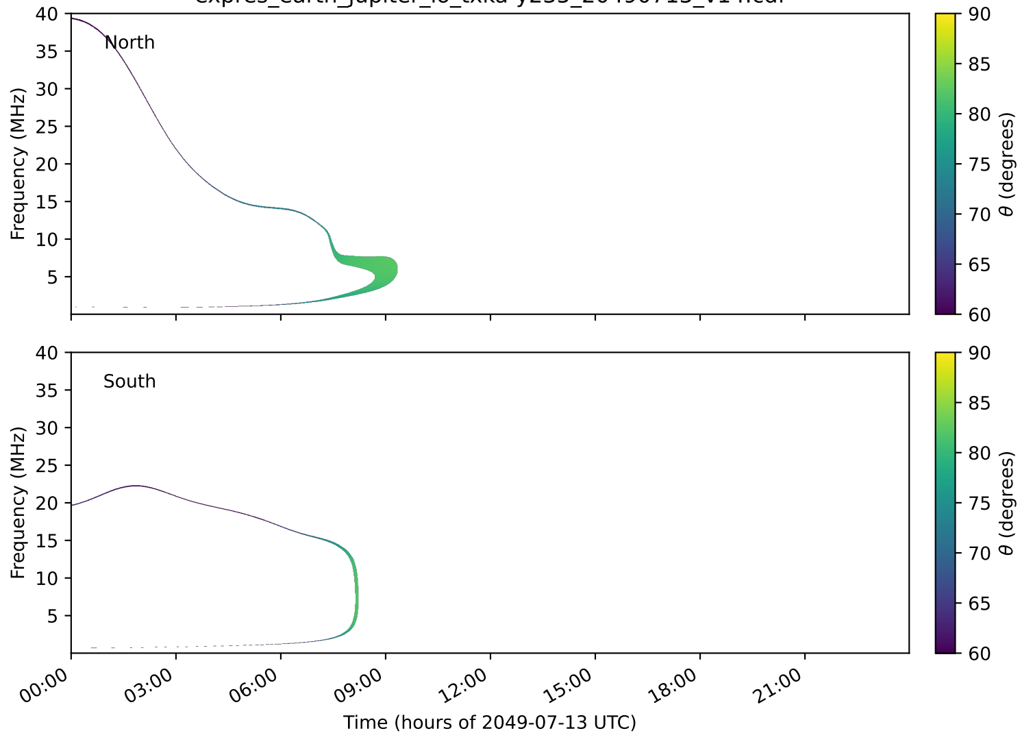
expres_earth_jupiter_io_txka-y235_20490713_v14.cdf
