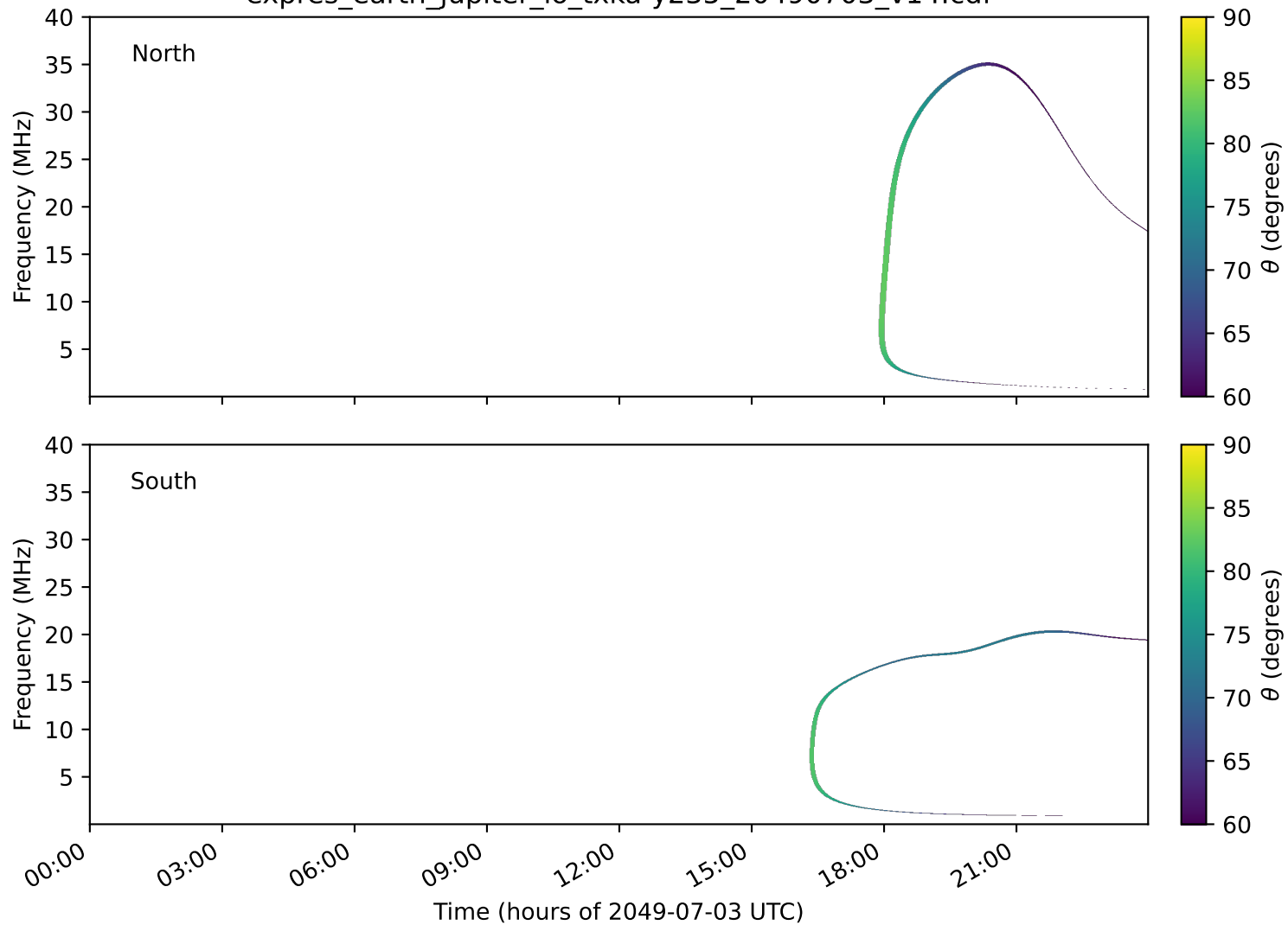
expres_earth_jupiter_io_txka-y235_20490703_v14.cdf
