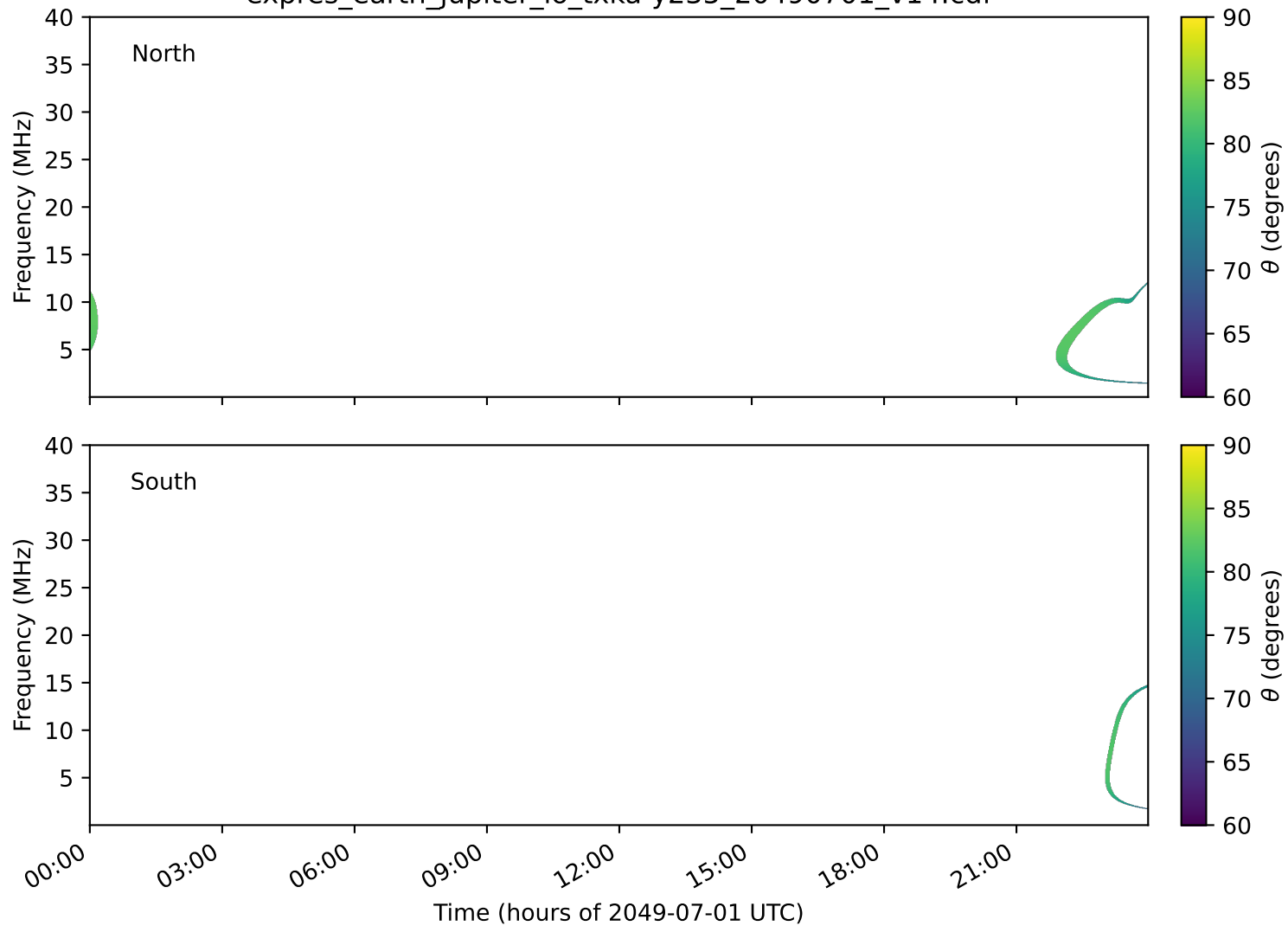
expres_earth_jupiter_io_txka-y235_20490701_v14.cdf
