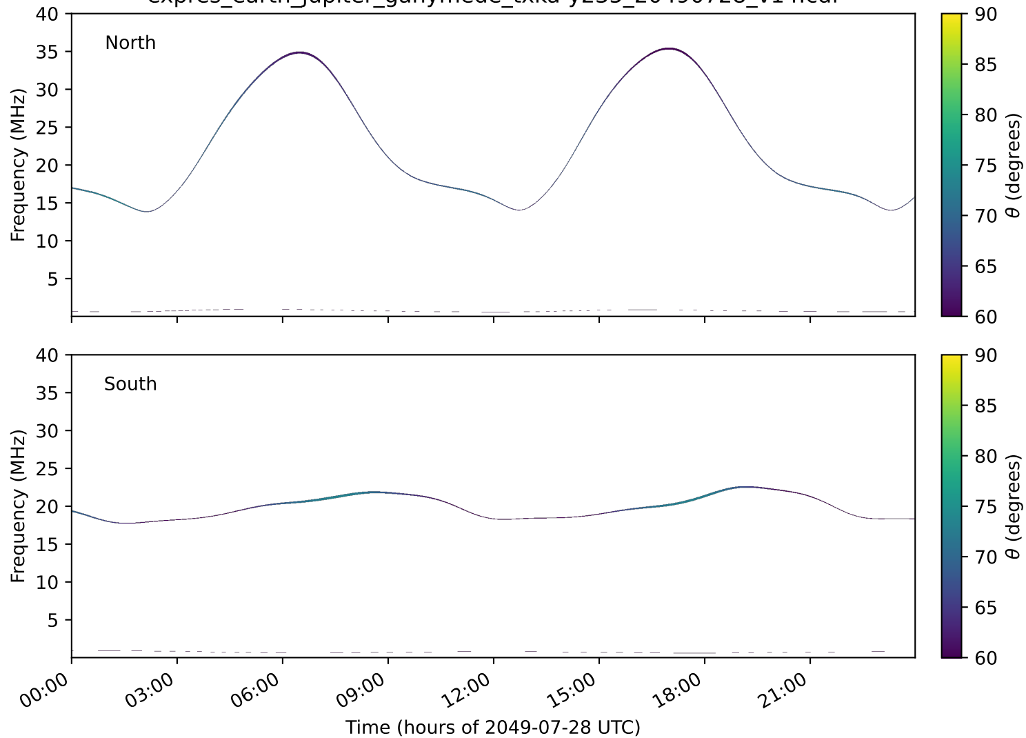
expres_earth_jupiter_ganymede_txka-y235_20490728_v14.cdf
