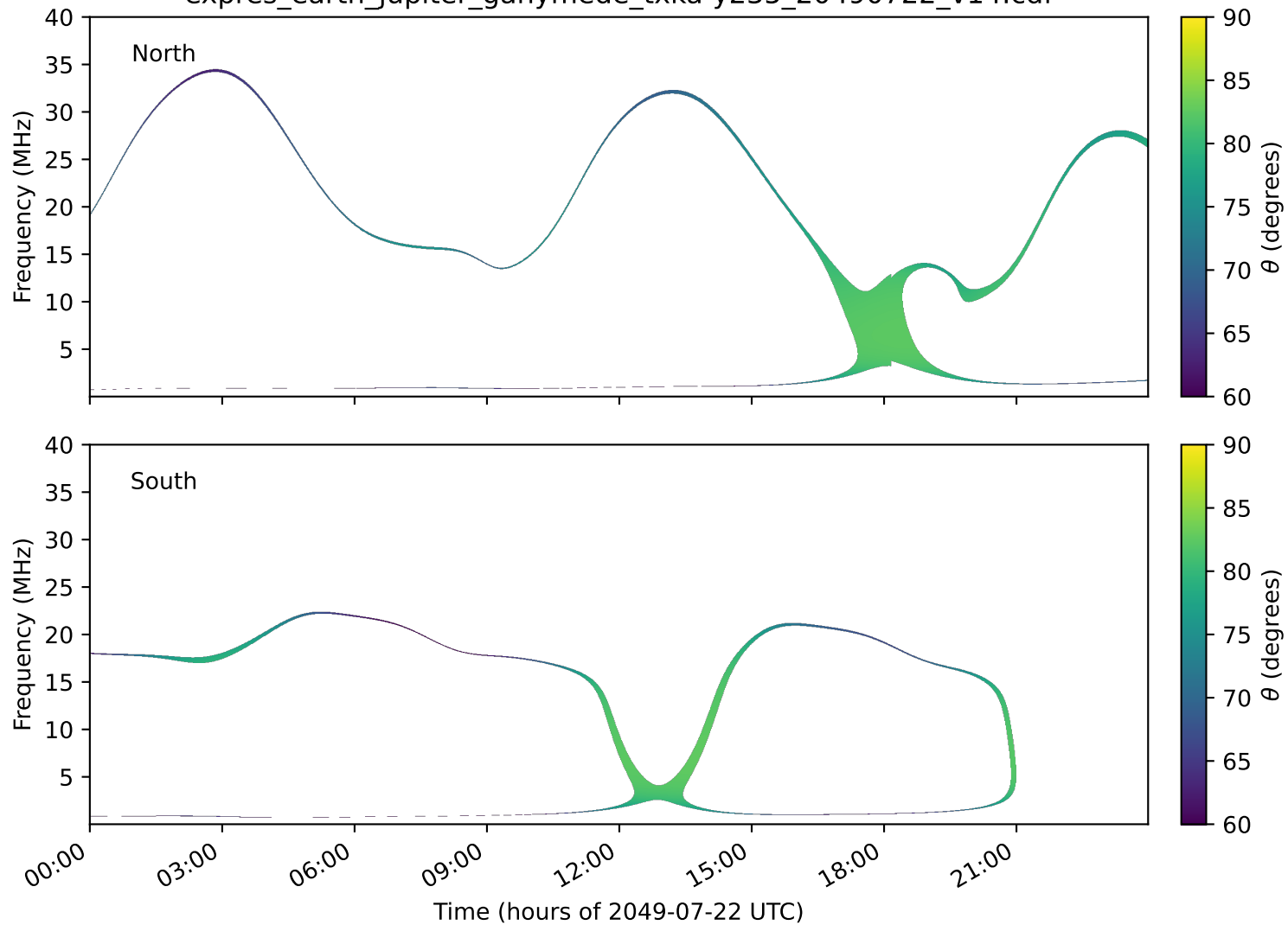
expres_earth_jupiter_ganymede_txka-y235_20490722_v14.cdf
