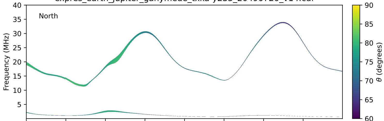
expres_earth_jupiter_ganymede_txka-y235_20490720_v14.cdf
