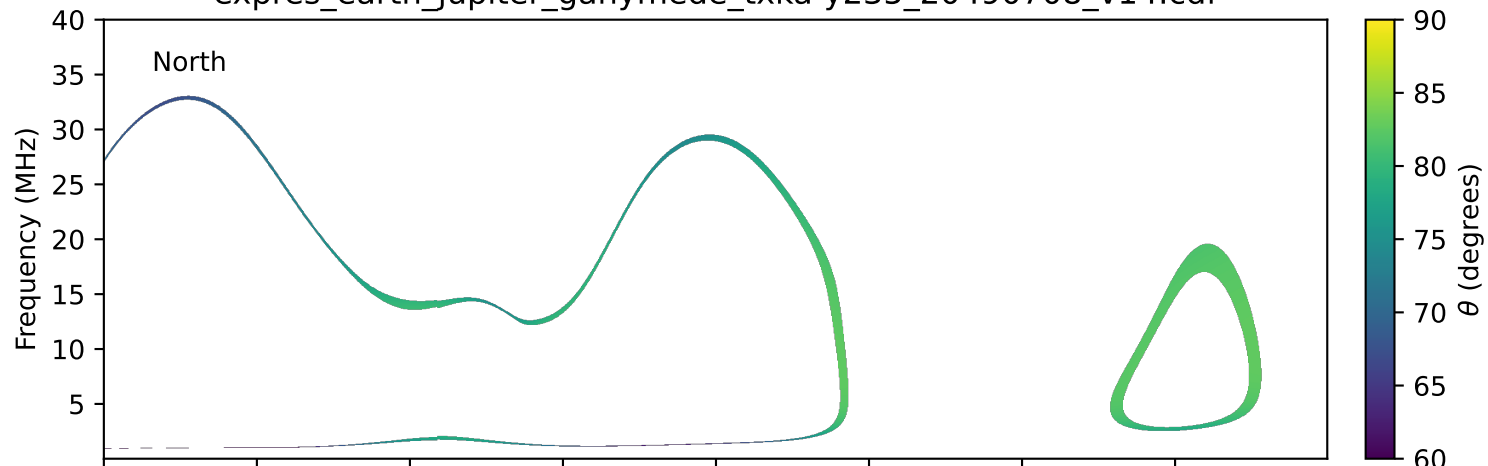
expres_earth_jupiter_ganymede_txka-y235_20490708_v14.cdf
