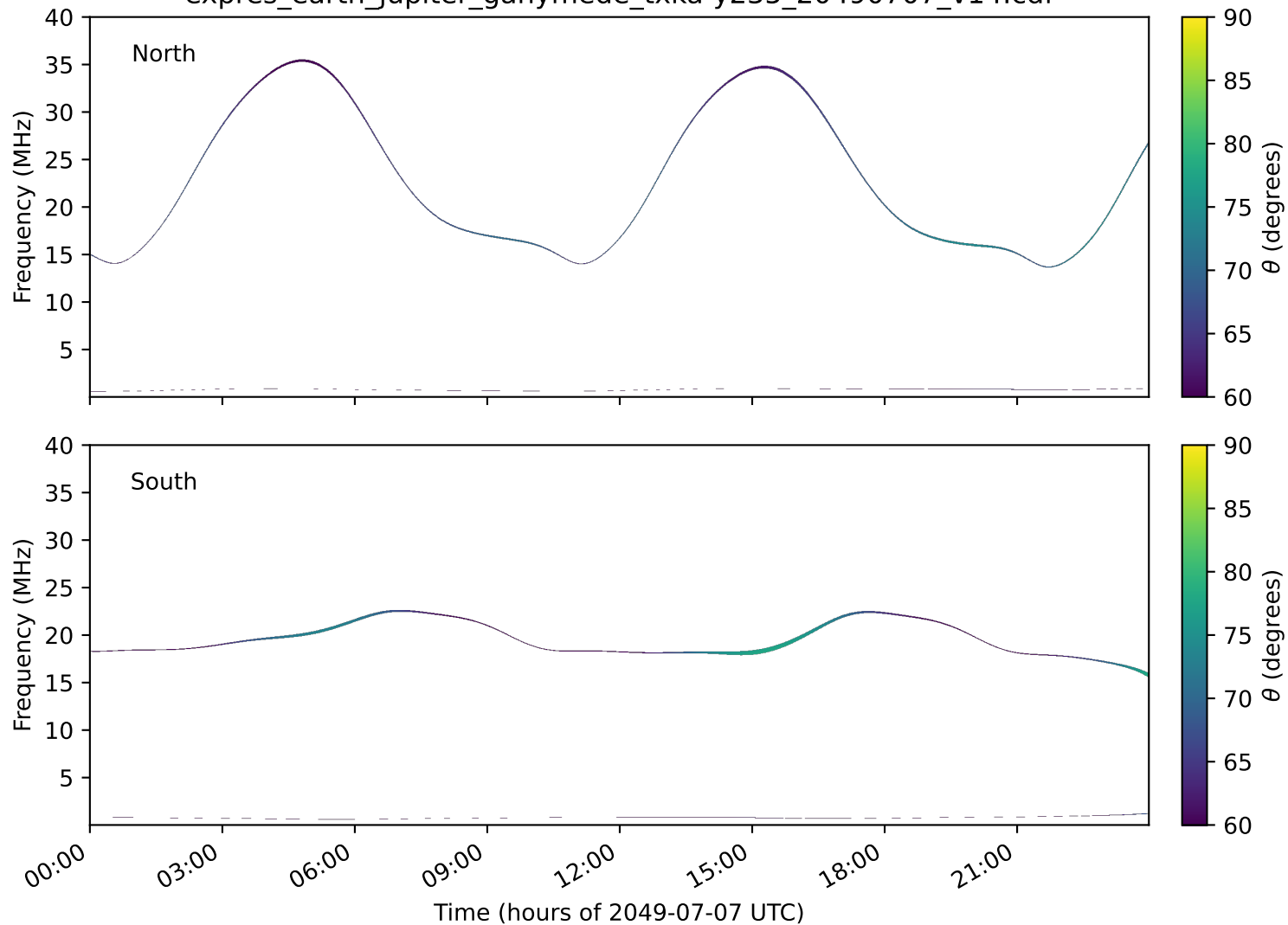
expres_earth_jupiter_ganymede_txka-y235_20490707_v14.cdf
