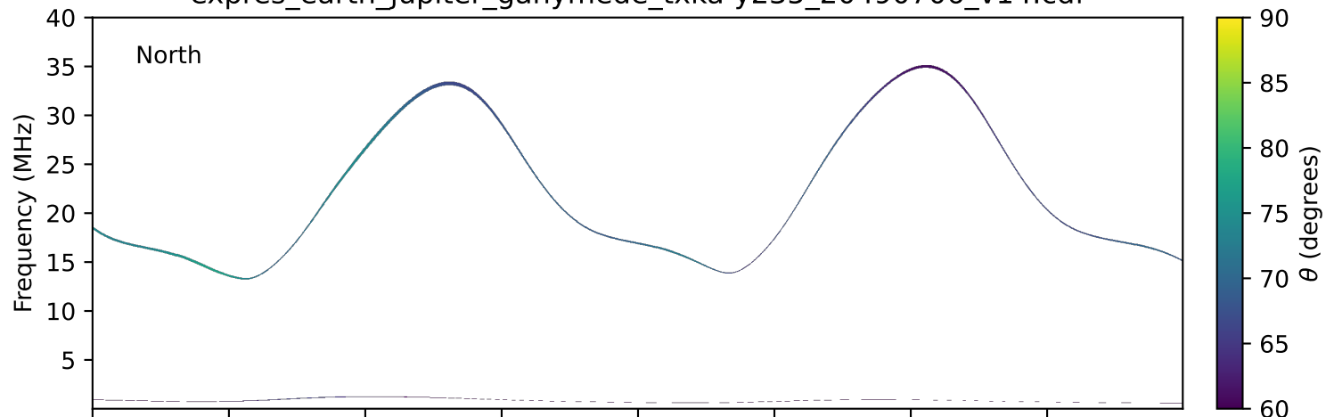
expres_earth_jupiter_ganymede_txka-y235_20490706_v14.cdf
