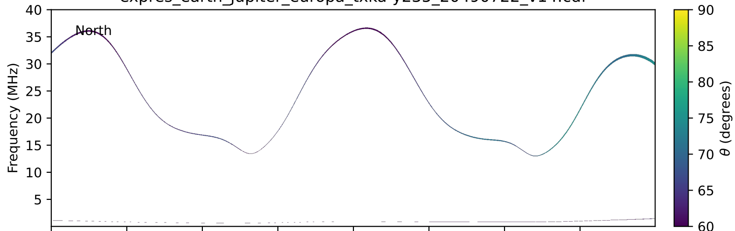
expres_earth_jupiter_europa_txka-y235_20490722_v14.cdf
