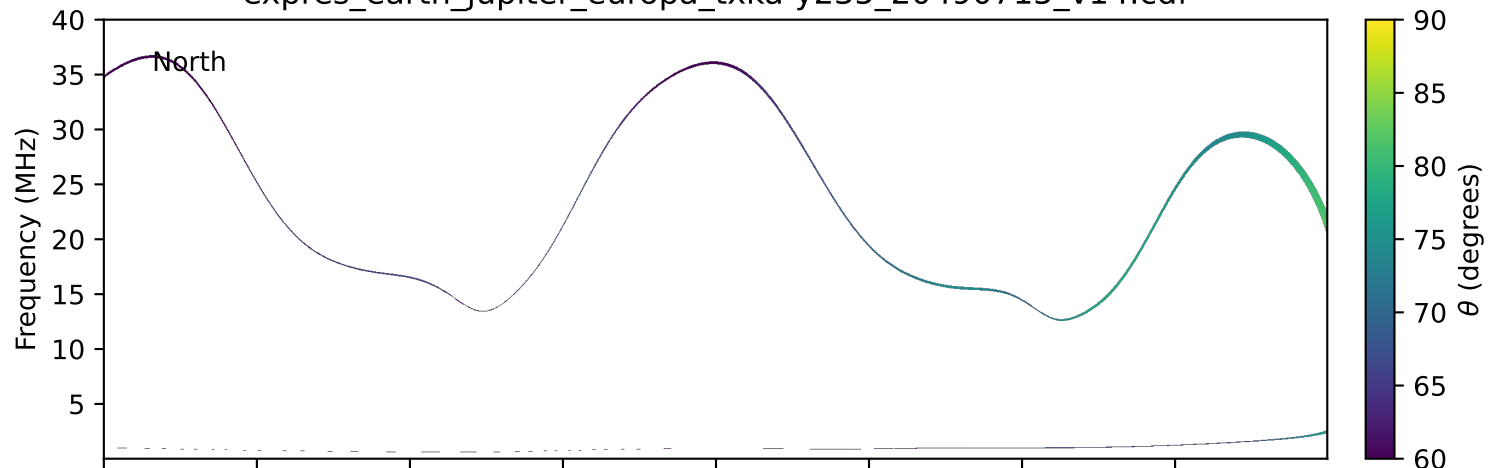
expres_earth_jupiter_europa_txka-y235_20490715_v14.cdf
