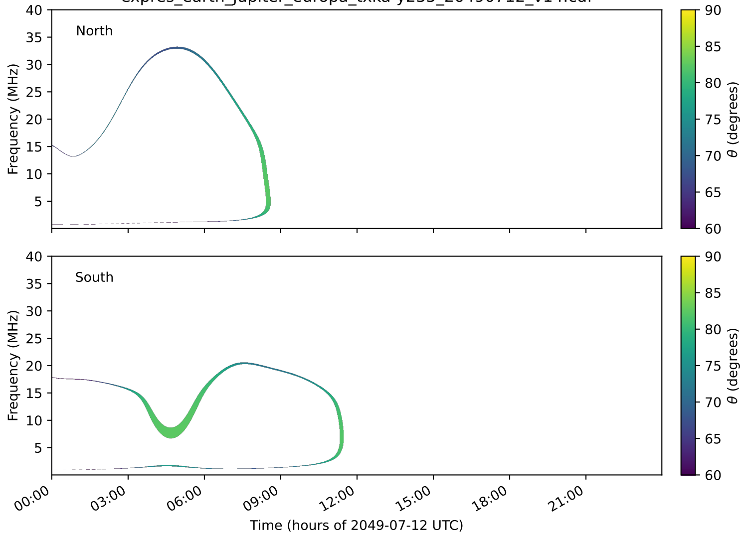
expres_earth_jupiter_europa_txka-y235_20490712_v14.cdf
