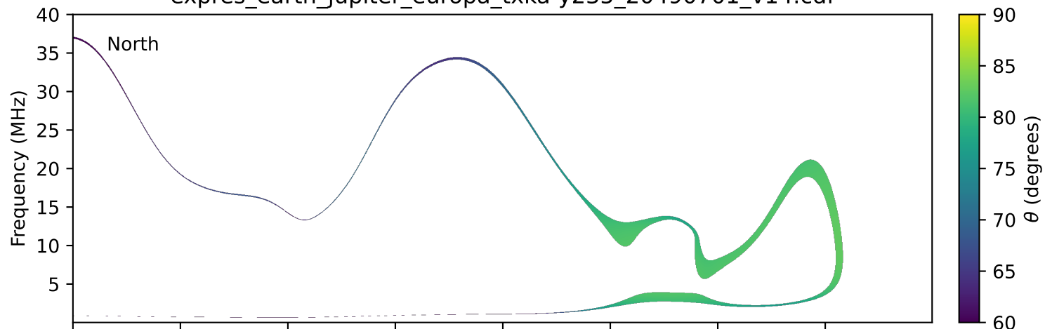
expres_earth_jupiter_europa_txka-y235_20490701_v14.cdf
