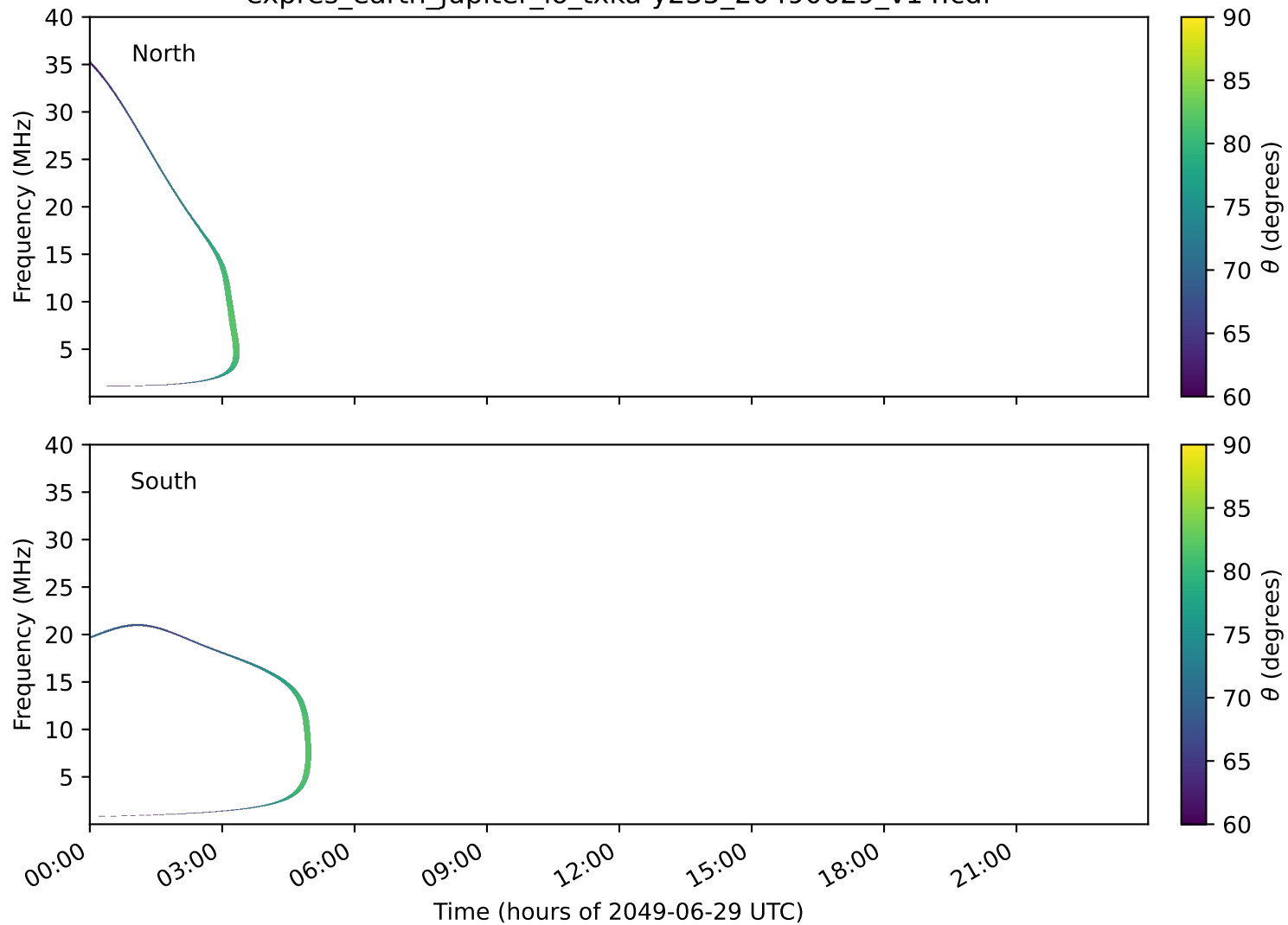
expres_earth_jupiter_io_txka-y235_20490629_v14.cdf
