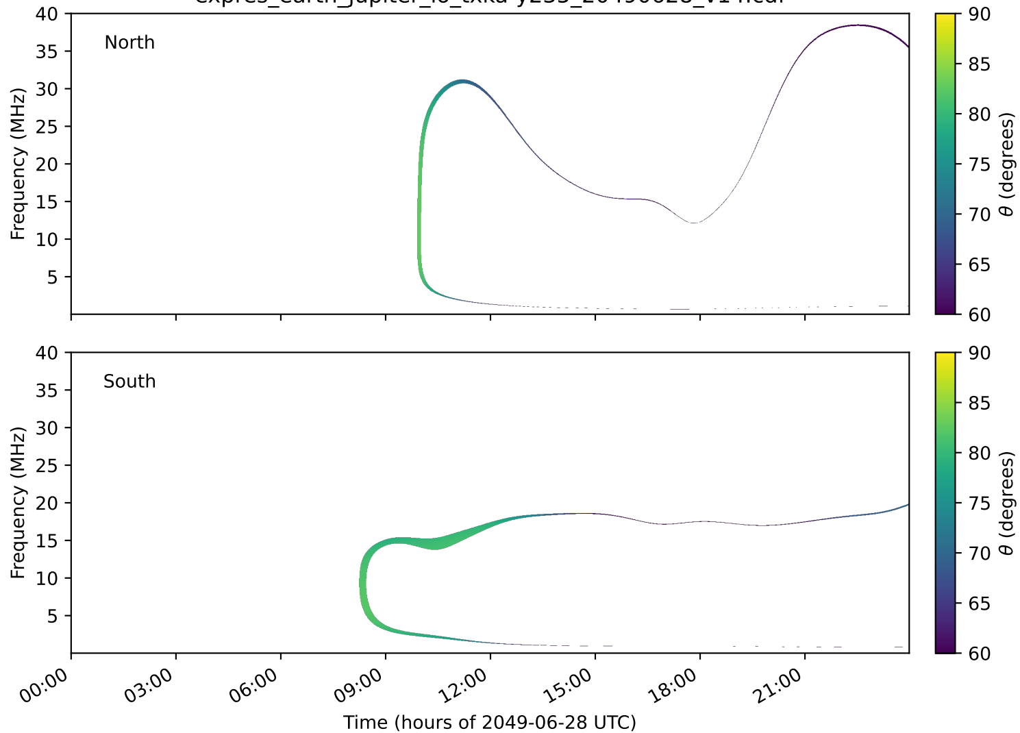
expres_earth_jupiter_io_txka-y235_20490628_v14.cdf
