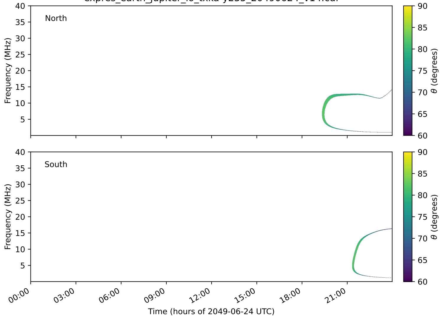
expres_earth_jupiter_io_txka-y235_20490624_v14.cdf
