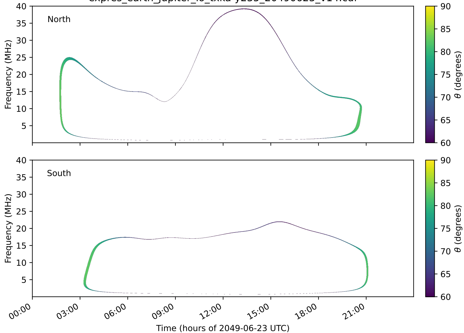
expres_earth_jupiter_io_txka-y235_20490623_v14.cdf
