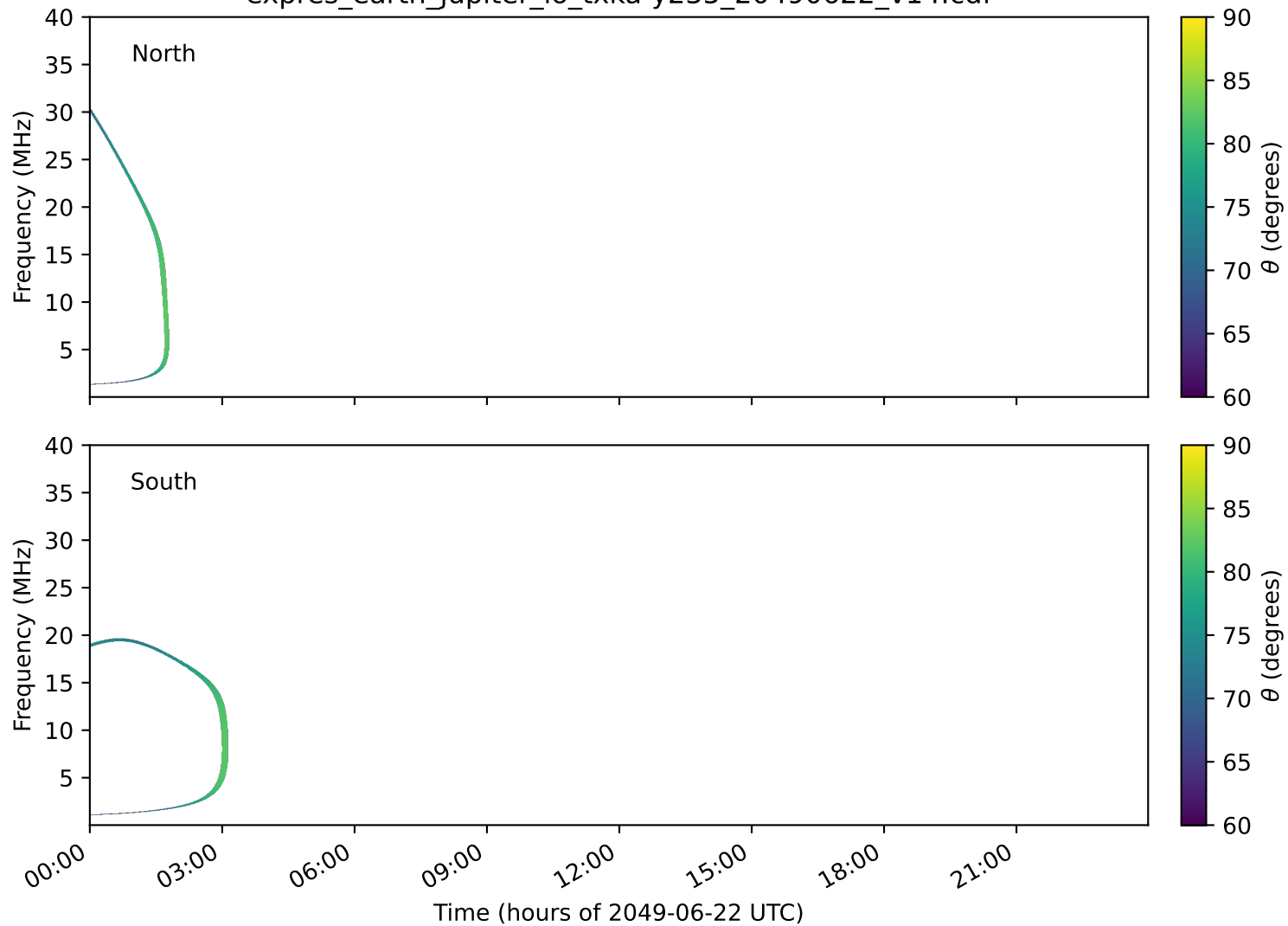
expres_earth_jupiter_io_txka-y235_20490622_v14.cdf
