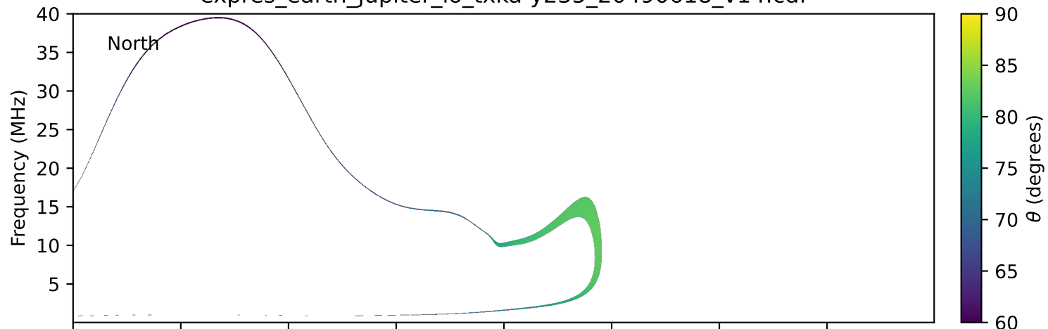
expres_earth_jupiter_io_txka-y235_20490618_v14.cdf
