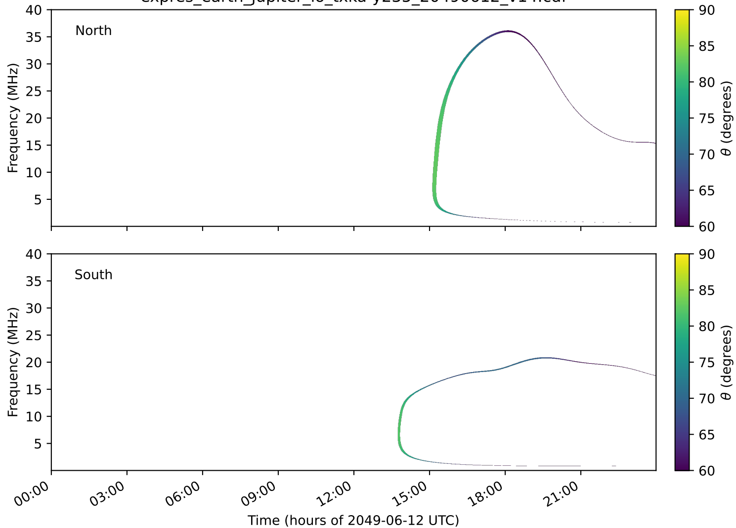
expres_earth_jupiter_io_txka-y235_20490612_v14.cdf
