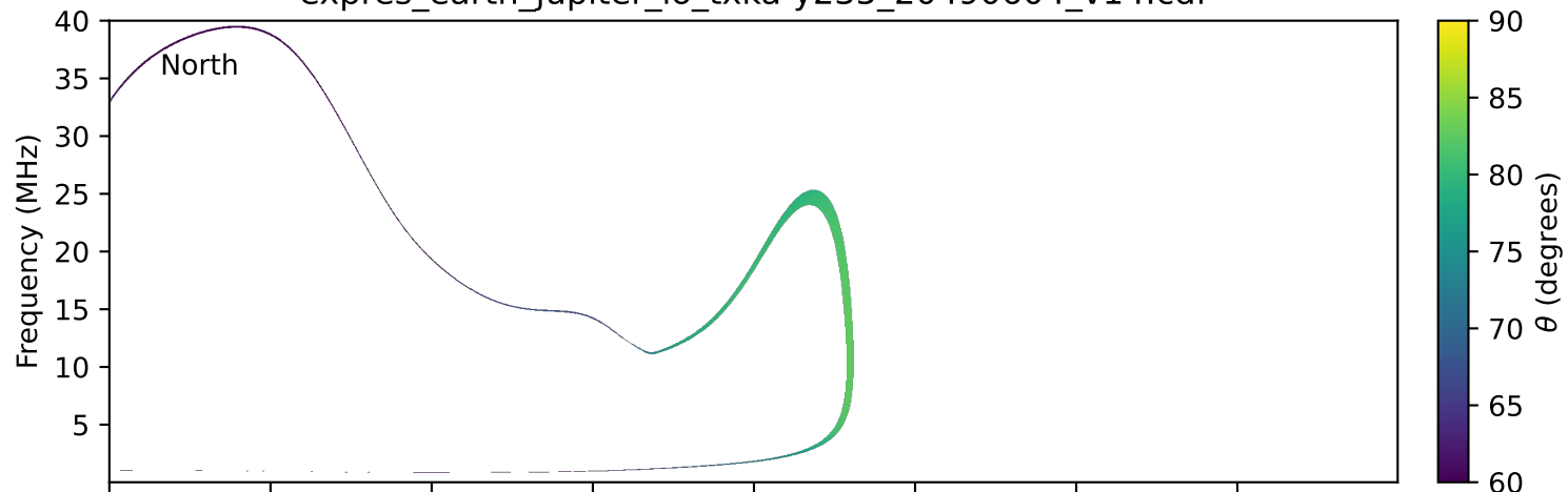
expres_earth_jupiter_io_txka-y235_20490604_v14.cdf
