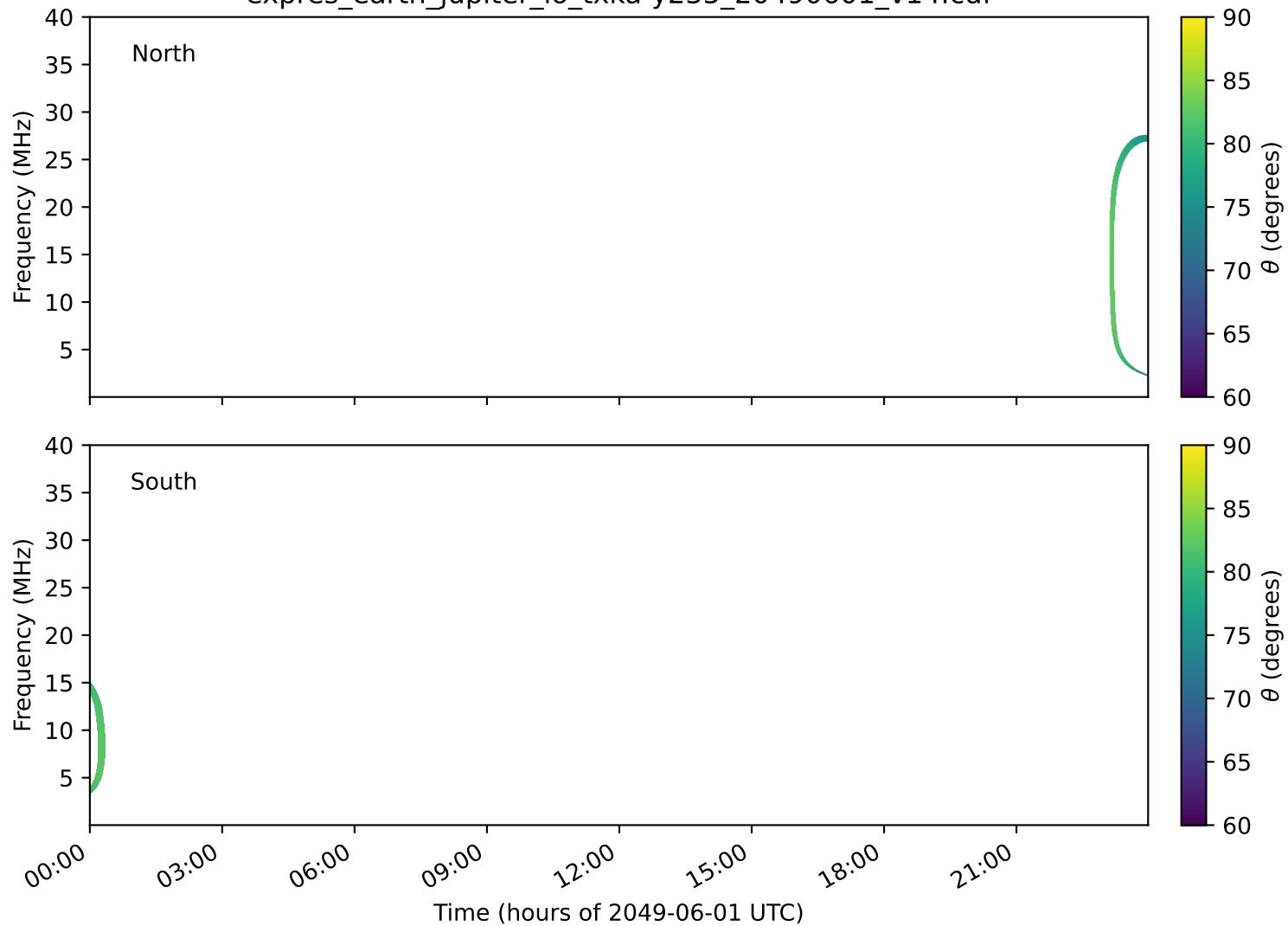
expres_earth_jupiter_io_txka-y235_20490601_v14.cdf
