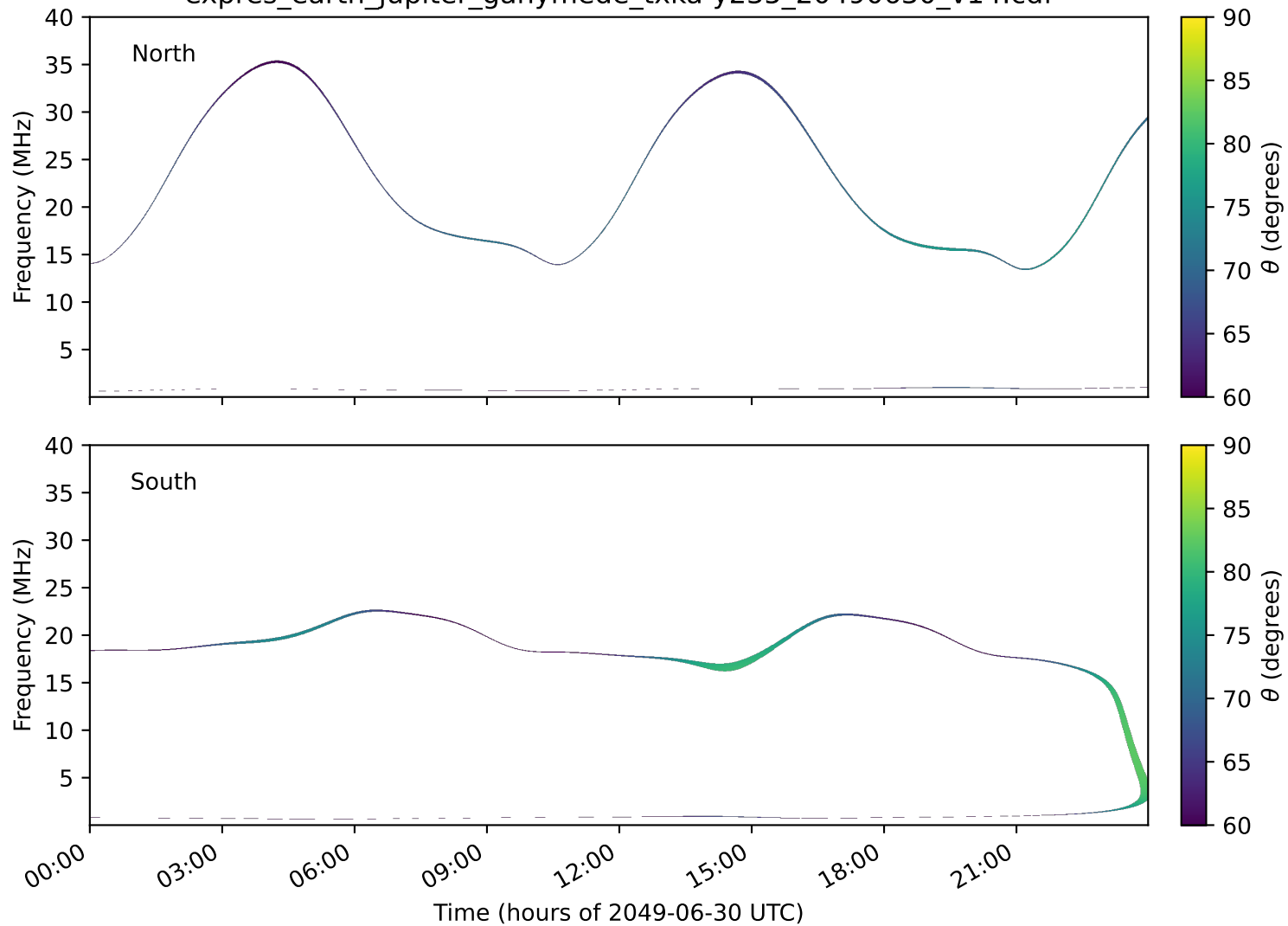
expres_earth_jupiter_ganymede_txka-y235_20490630_v14.cdf
