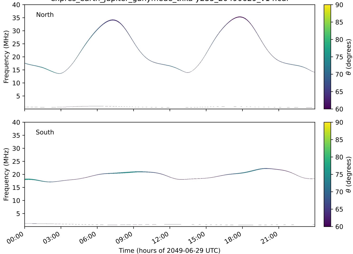
expres_earth_jupiter_ganymede_txka-y235_20490629_v14.cdf
