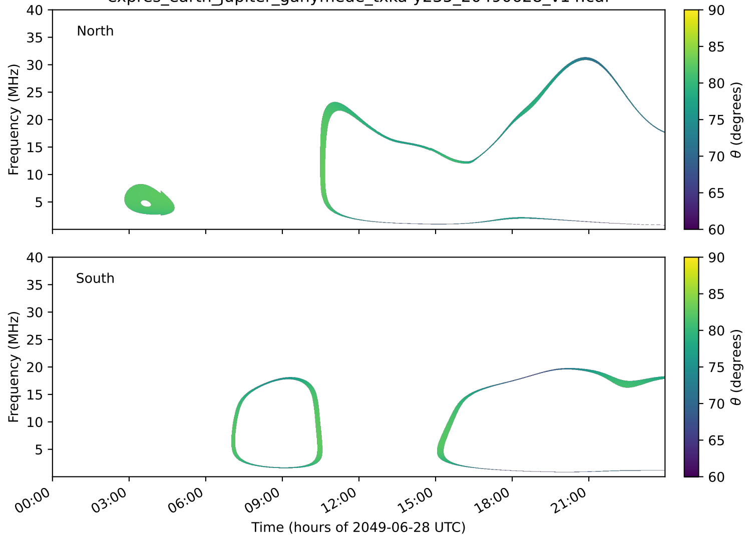
expres_earth_jupiter_ganymede_txka-y235_20490628_v14.cdf
