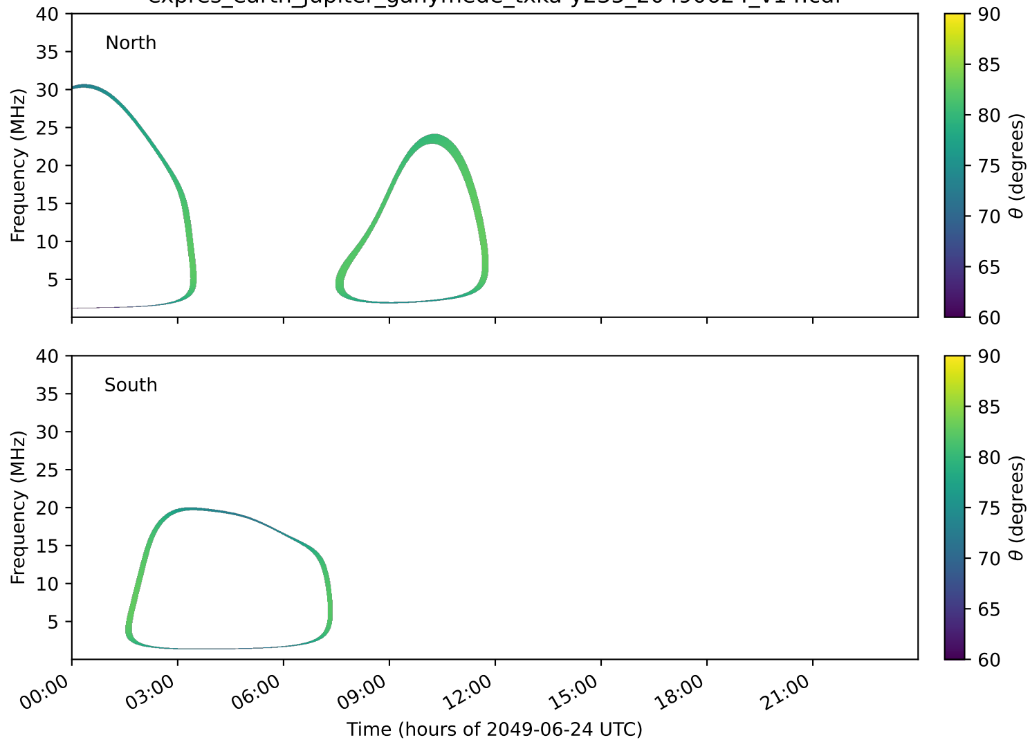
expres_earth_jupiter_ganymede_txka-y235_20490624_v14.cdf
