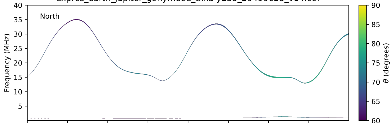
expres_earth_jupiter_ganymede_txka-y235_20490623_v14.cdf
