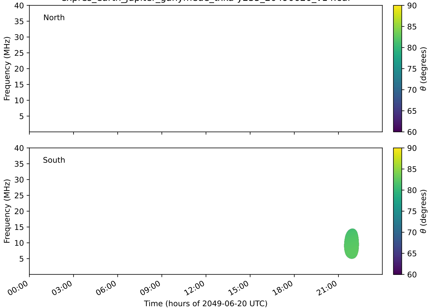
expres_earth_jupiter_ganymede_txka-y235_20490620_v14.cdf
