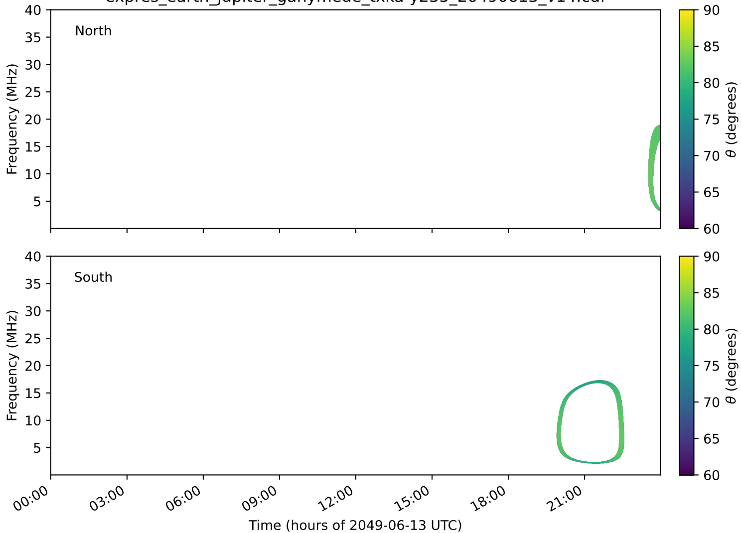
expres_earth_jupiter_ganymede_txka-y235_20490613_v14.cdf
