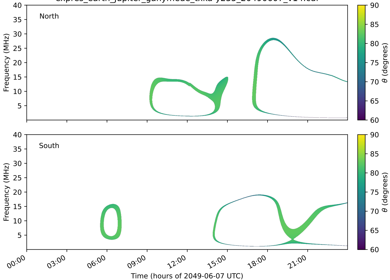
expres_earth_jupiter_ganymede_txka-y235_20490607_v14.cdf
