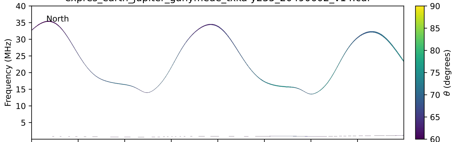
expres_earth_jupiter_ganymede_txka-y235_20490602_v14.cdf
